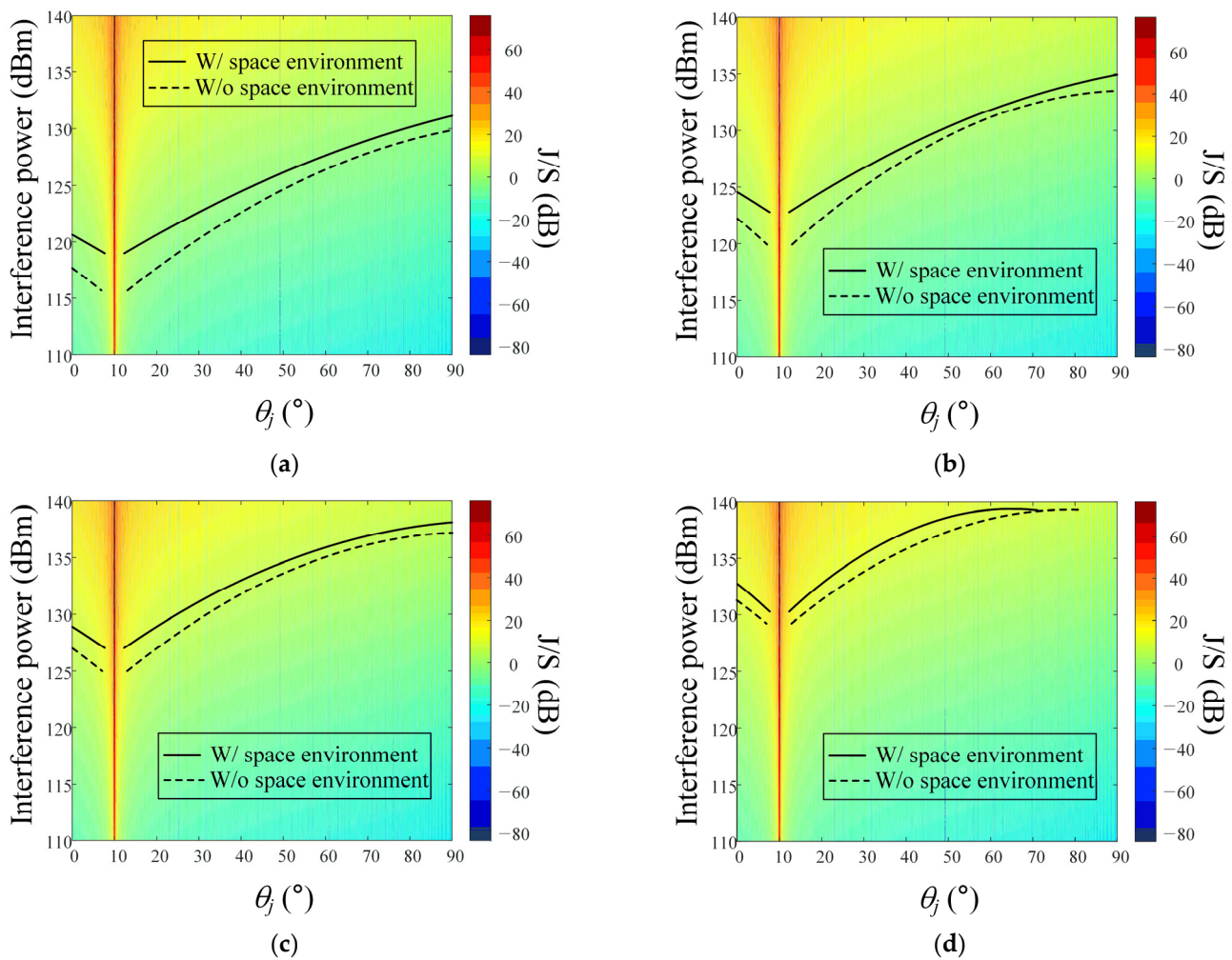
Figure 8. J/S according to the elevation angle \theta_j and the interference power at \theta_{gs} = 10^\circ : (a) J/S = 0 dB; (b) J/S = 5 dB; (c) J/S = 10 dB; (d) J/S = 15 dB.
