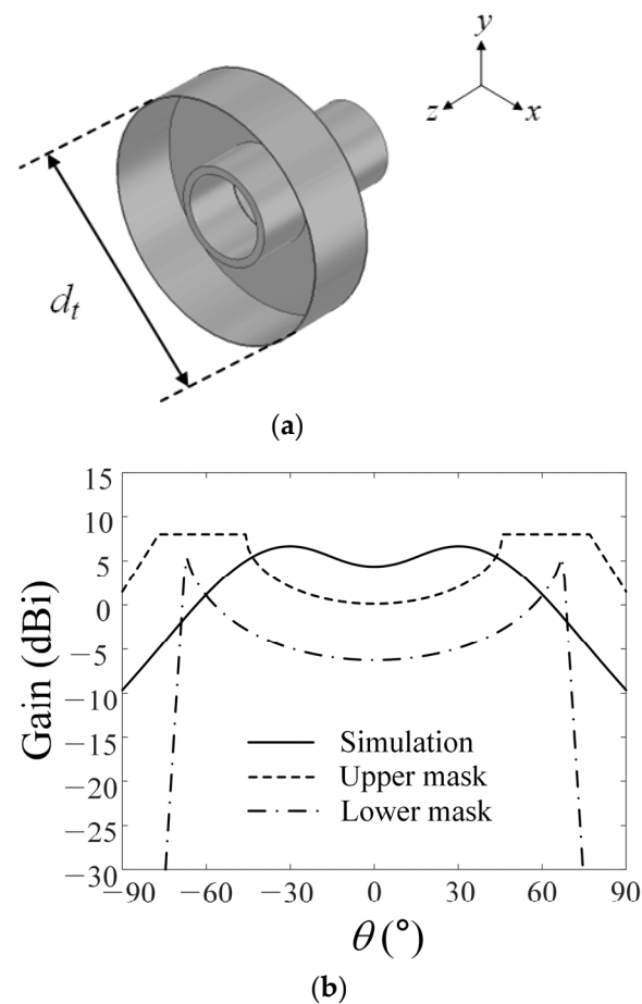
Figure 2. Transmitting antenna of the satellite and the far-zone radiation pattern: (a) transmitting antenna of the LEO satellite; (b) radiation pattern and requirement masks.
