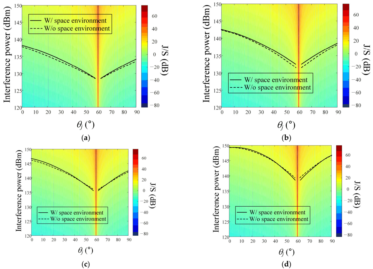
Figure 9. J/S according to the elevation angle \theta_j and the interference power at \theta_{gs} = 60^\circ : (a) J/S = 0 dB; (b) J/S = 5 dB; (c) J/S = 10 dB; (d) J/S = 15 dB.
