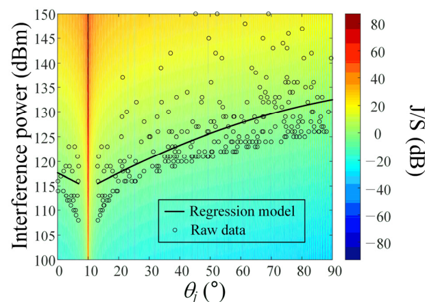
Figure 7. J/S according to the elevation angle \theta_j and the interference power. “○” is when J/S = 0 dB, and the solid line is the regression model.
