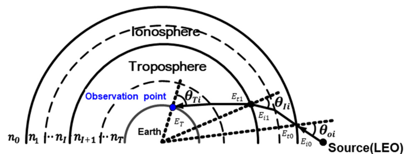
Figure 4. Geometrical optics model in a space environment.
