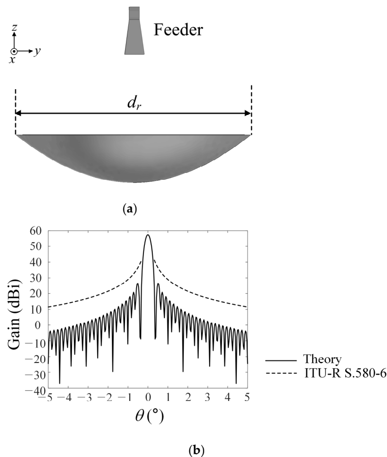
Figure 3. Receiving antenna of the ground station and the far-zone radiation pattern: (a) receiving antenna of the ground station; (b) far-zone radiation pattern of the ground station.
