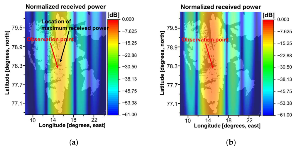
Figure 6. Normalized received power at \theta_{gs} = 10^\circ : (a) in free space; (b) in the space environment.
