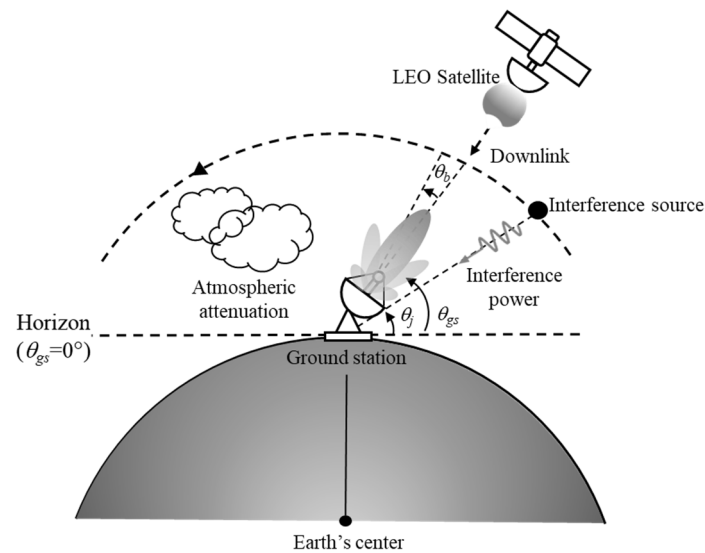
Figure 1. Conceptual figure of the LEO downlink scenario in interference situations.
